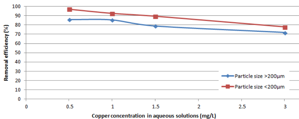
Fig. 1. Adsorption percent of cooper by two fractions of coffee grounds
